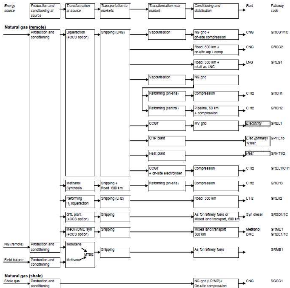
Figura 4. Natural Gas Pathways JEC - Joint Research Centre-EUCAR-CONCAWE collaboration, Well-to-Wheels analysis of future automotive fuels and powertrains in the European context. WELL-TO-TANK (WTT) Report. Version 4 a , January 2014
